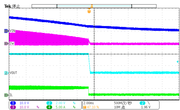
Figure 14. Power down(Iload=3.5A)
